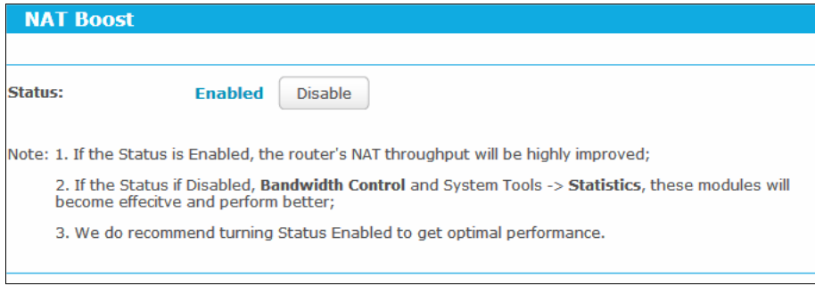
Figure 5-49 NAT Boost
