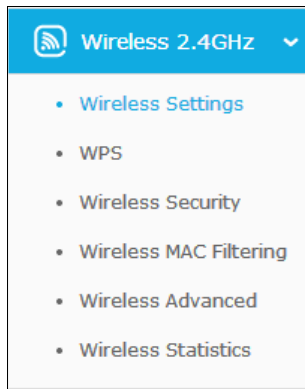
Figure 5-12 Wireless menu
