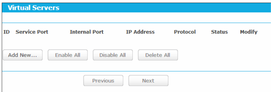
Figure 5-51 Virtual Servers
