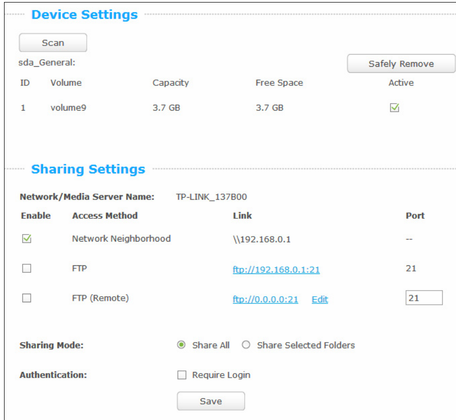
Figure 4-9 File Sharing
