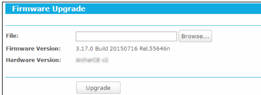
Figure 5-107 Firmware Upgrade
