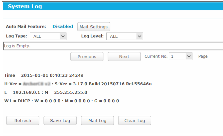
Figure 5-112 System Log
