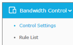
Figure 5-83 Bandwidth Control
